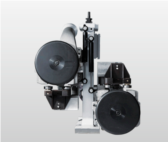
MF21 multi-trimming unit
