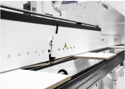
Belt-type top roll pressure The top roll pressure element made of steel with double V-belt provides the basis for the highest quality because your workpieces are optimally clamped for processing.
